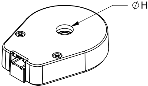
H-OPTION COVER (HOLE FOR SHAFT LENGTHS OVER .750 [19.05])
