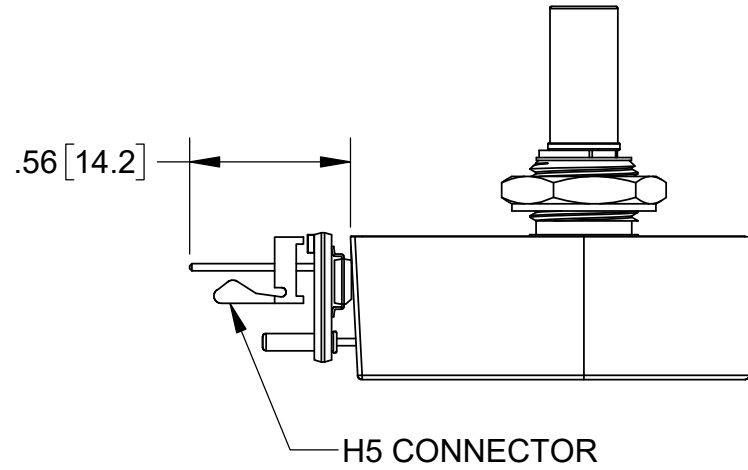
SHOWN MOUNTED ON AN S1 ENCODER
